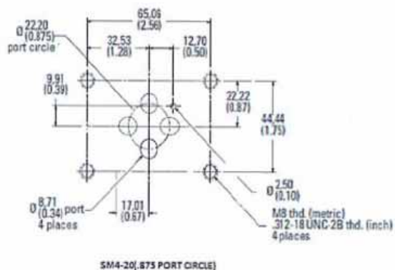
SM4-20 (.875 PORT CIRCLE)
